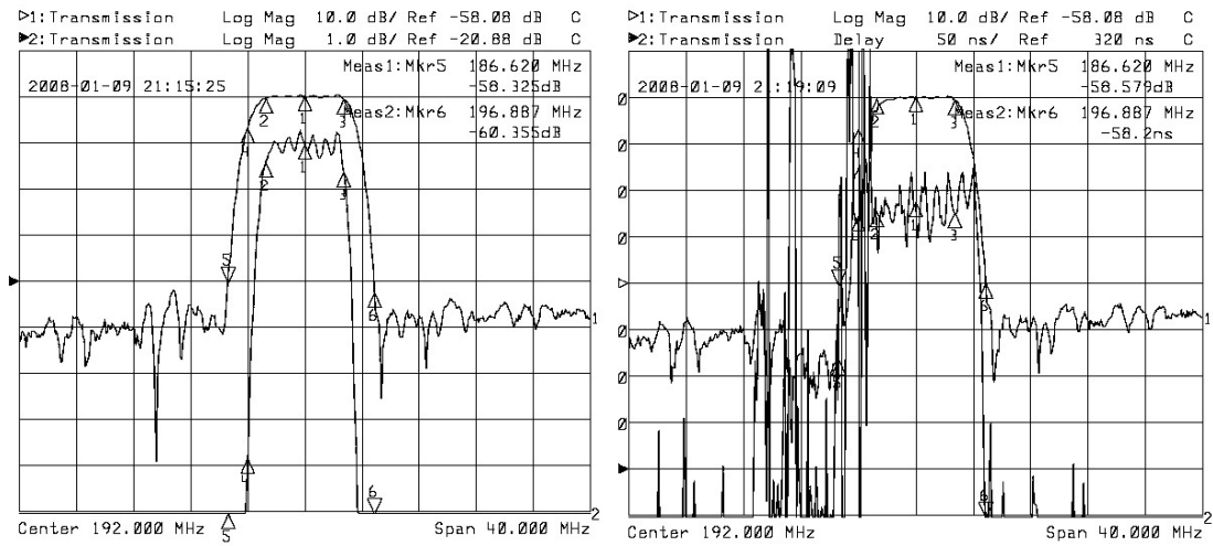
Horizontal: 4MHz/Div Vertical: 1dB/Div&10dB/Div
