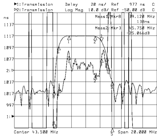
Horizontal: 2MHz/Div Vertical: 20nsec/Div&10dB/Div
