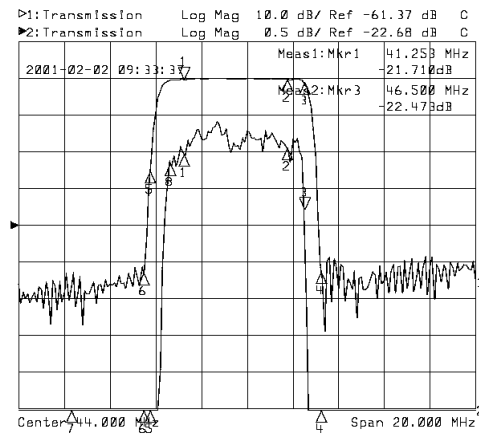
Horizontal: 2MHz/Div Vertical: 0.5dB/Div&10dB/Div
