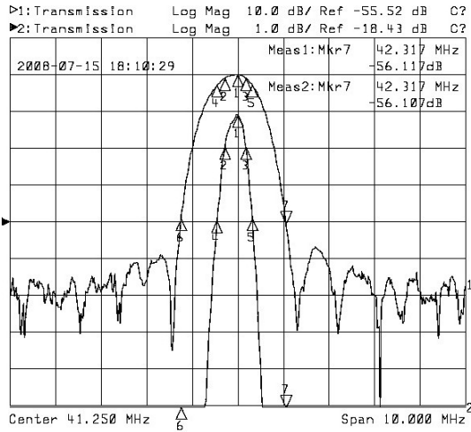
Horizontal: 1MHz/Div Vertical: 1dB/Div&10dB/Div
