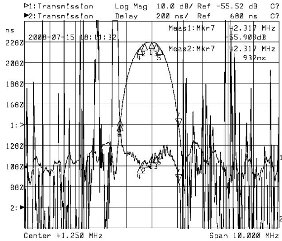
Horizontal: 1MHz/Div Vertical: 200nsec/Div&10dB/Div
