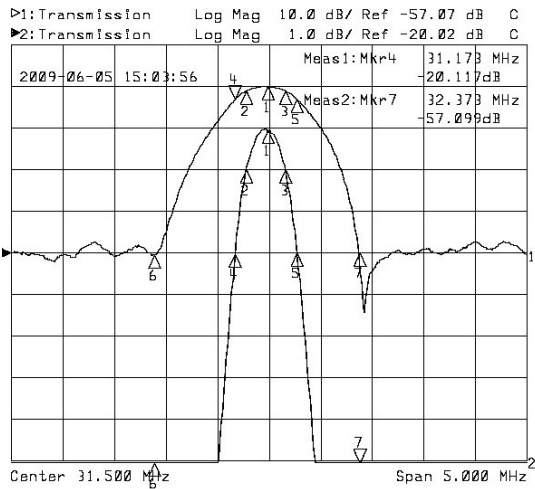
Horizontal: 0.5MHz/Div Vertical: 1dB/Div&10dB/Div
