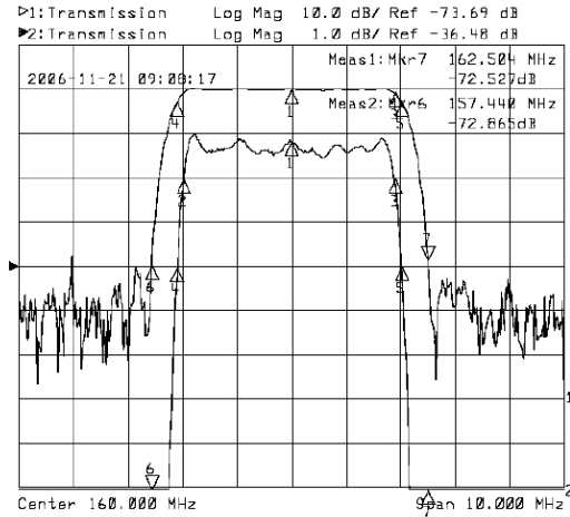
Horizontal: 1.0MHz/Div Vertical: 1dB/Div&10dB/Div
