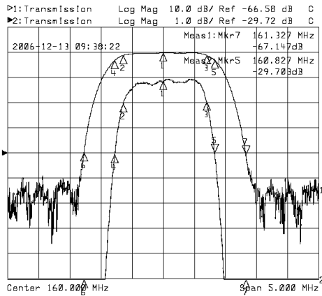
Horizontal: 0.5MHz/Div Vertical: 1dB/Div&10dB/Div
