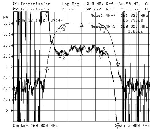
Horizontal: 0.5MHz/Div Vertical: 100nsec/Div&10dB/Div
