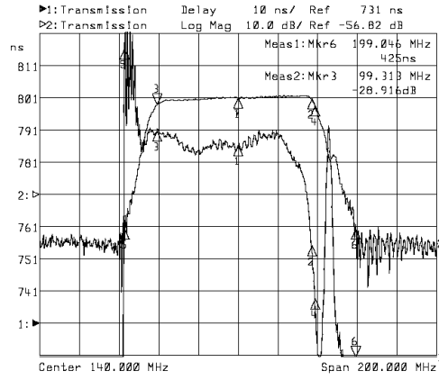
Horizontal: 20MHz/Div Vertical: 10nsec/Div&10dB/Div
