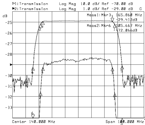
Horizontal: 10MHz/Div Vertical: 1dB/Div&10dB/Div
