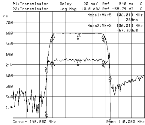
Horizontal: 14MHz/Div Vertical: 20nsec/Div&10dB/Div
