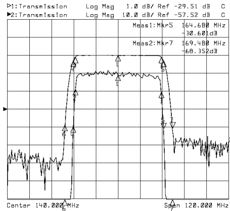
Horizontal: 12MHz/Div Vertical: 1dB/Div&10dB/Div
