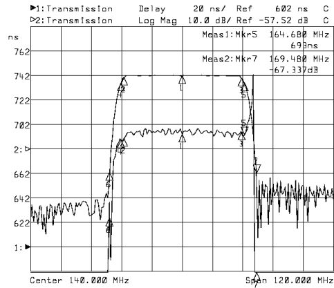
Horizontal: 12MHz/Div Vertical: 20nsec/Div&10dB/Div
