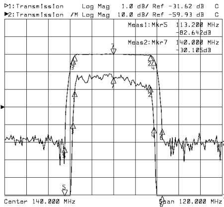
Horizontal: 12MHz/Div Vertical: 1dB/Div&10dB/Div
