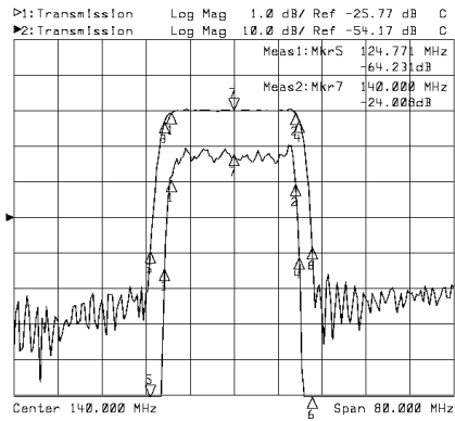
Horizontal: 8MHz/Div Vertical: 1dB/Div&10dB/Div
