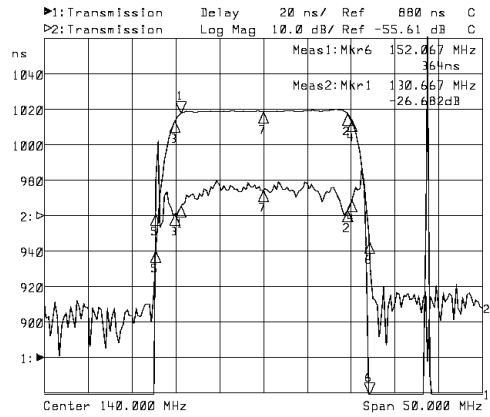
Horizontal: 5MHz/Div Vertical: 20nsec/Div&10dB/Div
