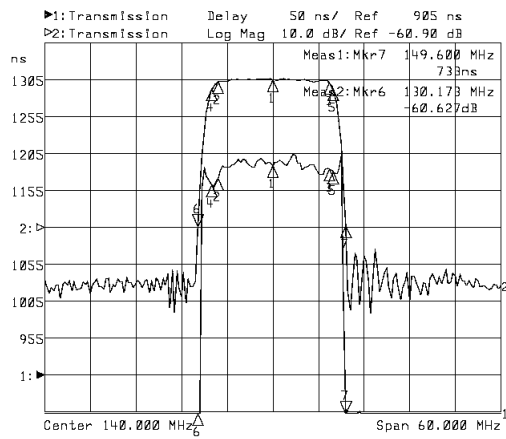
Horizontal: 6MHz/Div Vertical: 50nsec/Div&10dB/Div
