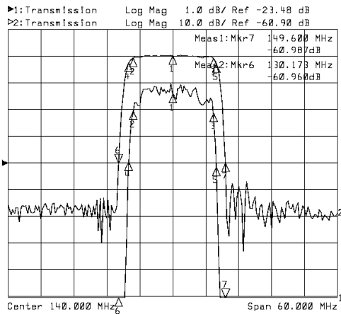
Horizontal: 6MHz/Div Vertical: 1dB/Div&10dB/Div
