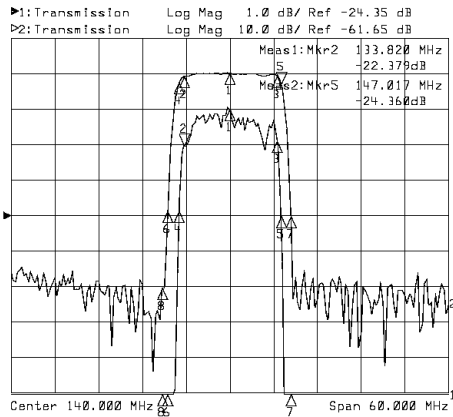
Horizontal: 6MHz/Div Vertical: 1dB/Div&10dB/Div
