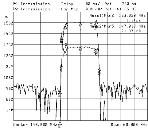
Horizontal: 6MHz/Div Vertical: 100nsec/Div&10dB/Div
