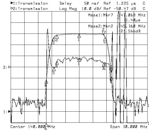
Horizontal: 3.0MHz/Div Vertical: 50nsec/Div&10dB/Div
