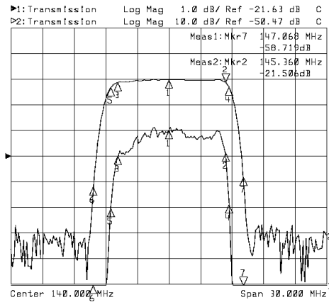
Horizontal: 3.0MHz/Div Vertical: 1dB/Div&10dB/Div
