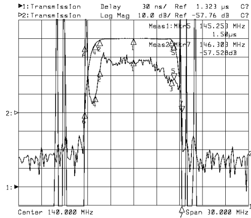
Horizontal: 3.0MHz/Div Vertical: 30nsec/Div&10dB/Div
