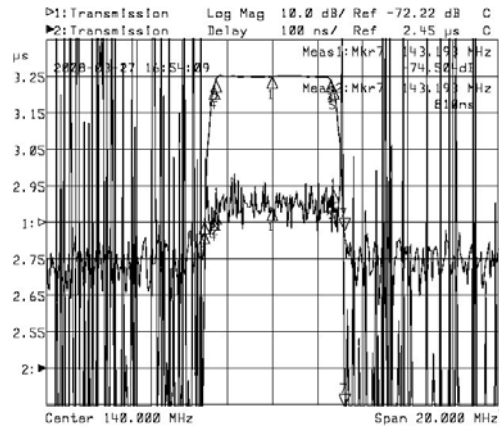
Horizontal: 1MHz/Div
