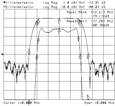
Horizontal: 1.0MHz/Div Vertical: 1dB/Div&10dB/Div
