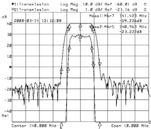
Horizontal: 1MHz/Div Vertical: 1dB/Div&10dB/Div
