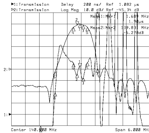
Horizontal: 0.6MHz/Div Vertical: 200nsec/Div&10dB/Div
