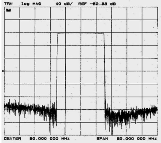
Horizontal: 8MHz/Div Vertical: 10dB/Div
