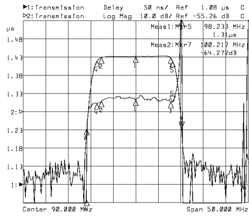
Horizontal: 5MHz/Div Vertical: 50nsec/Div&10dB/Div
