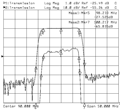
Horizontal: 5MHz/Div Vertical: 1dB/Div&10dB/Div
