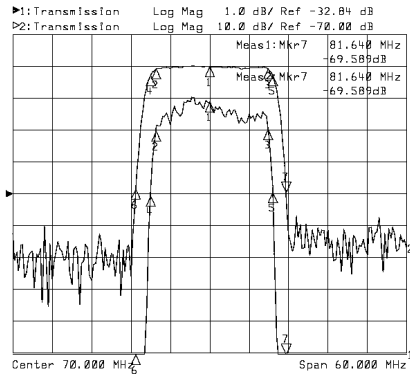
Horizontal: 6MHz/Div Vertical: 1dB/Div&10dB/Div
