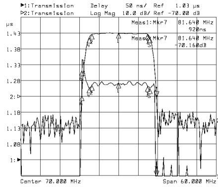
Horizontal: 6MHz/Div Vertical: 50nsec/Div&10dB/Div
