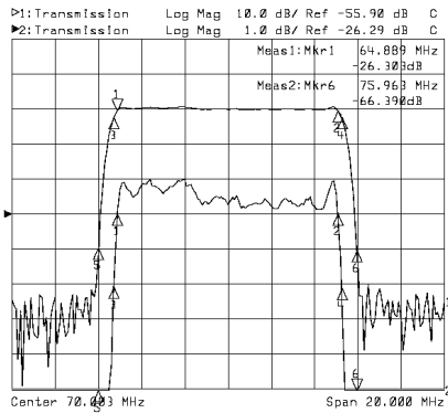
Horizontal: 2MHz/Div Vertical: 1dB/Div&10dB/Div
