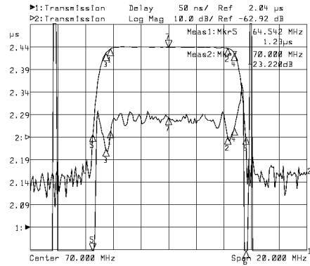
Horizontal: 2MHz/Div Vertical: 50nsec/Div & 10dB/Div
