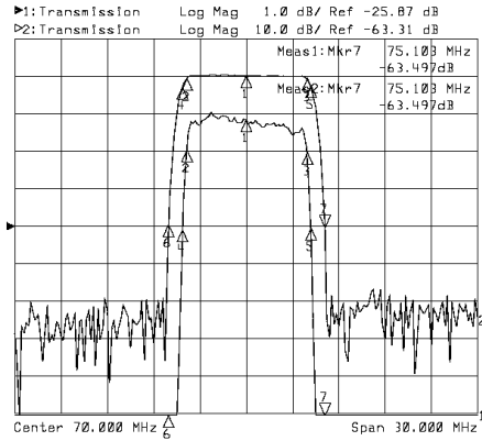
Horizontal: 3MHz/Div Vertical: 1dB/Div & 10dB/Div
