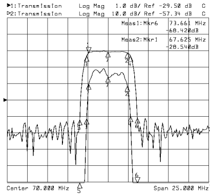
Horizontal: 2.5MHz/Div Vertical: 1dB/Div&10dB/Div
