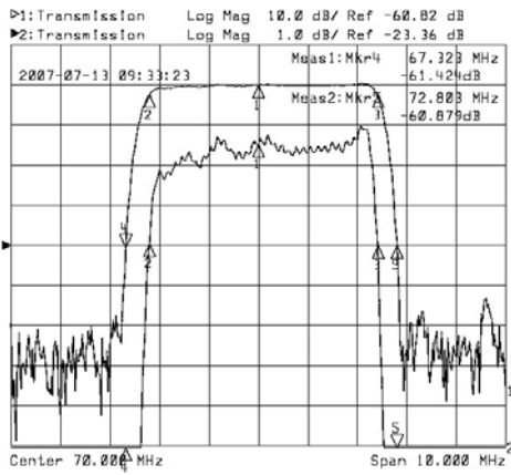
Horizontal: 1MHz/Div Vertical: 1dB/Div&10dB/Div
