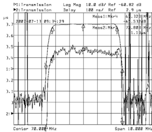
Horizontal: 1MHz/Div Vertical: 100ns/Div&10dB/Div
