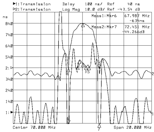
Horizontal: 2MHz/Div Vertical: 100ns/Div&10dB/Div
