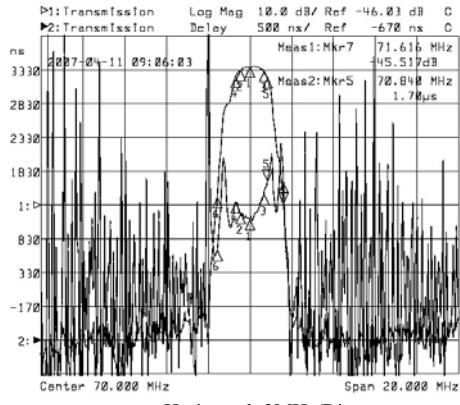
Horizontal: 2MHz/Div Vertical: 500ns/Div&10dB/Div
