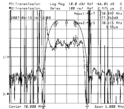
Horizontal: 0.5MHz/Div Vertical: 100ns/Div&10dB/Div
