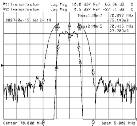
Horizontal: 0.5MHz/Div Vertical: 0.5dB/Div&10dB/Div
