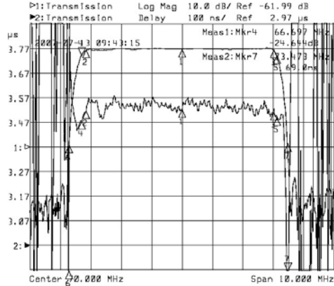
Horizontal: 1MHz/Div Vertical: 100ns/Div&10dB/Div
