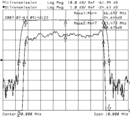
Horizontal: 1MHz/Div Vertical: 1dB/Div&10dB/Div
